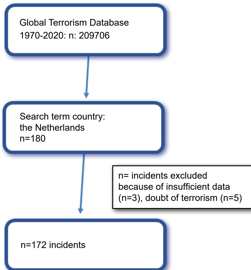
Figure 1: PRISMA.
